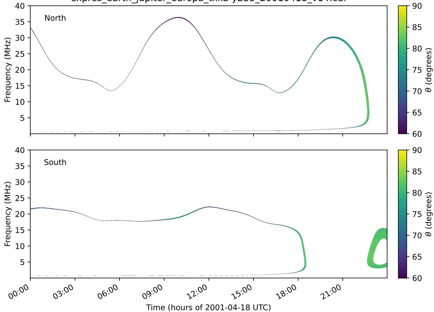
expres_earth_jupiter_europa_txka-y235_20010418_v14.cdf
