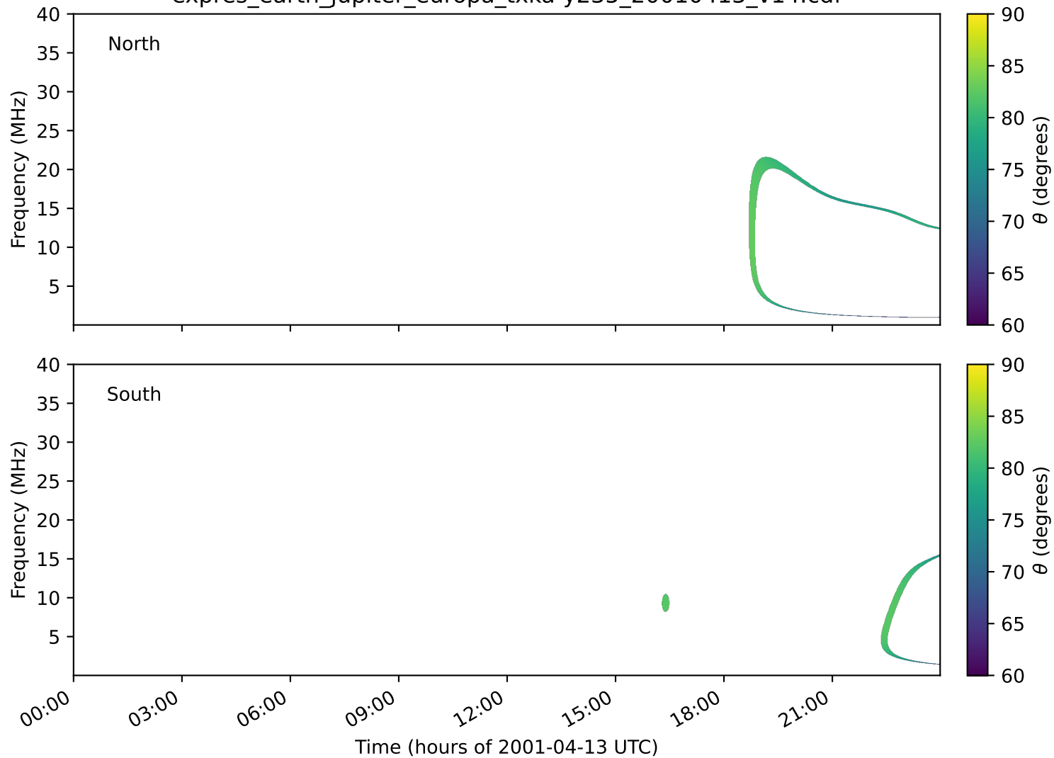
expres_earth_jupiter_europa_txka-y235_20010413_v14.cdf
