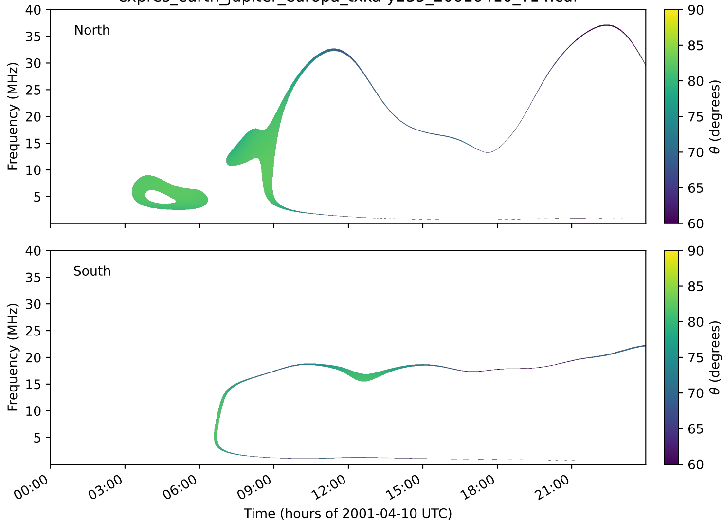
expres_earth_jupiter_europa_txka-y235_20010410_v14.cdf
