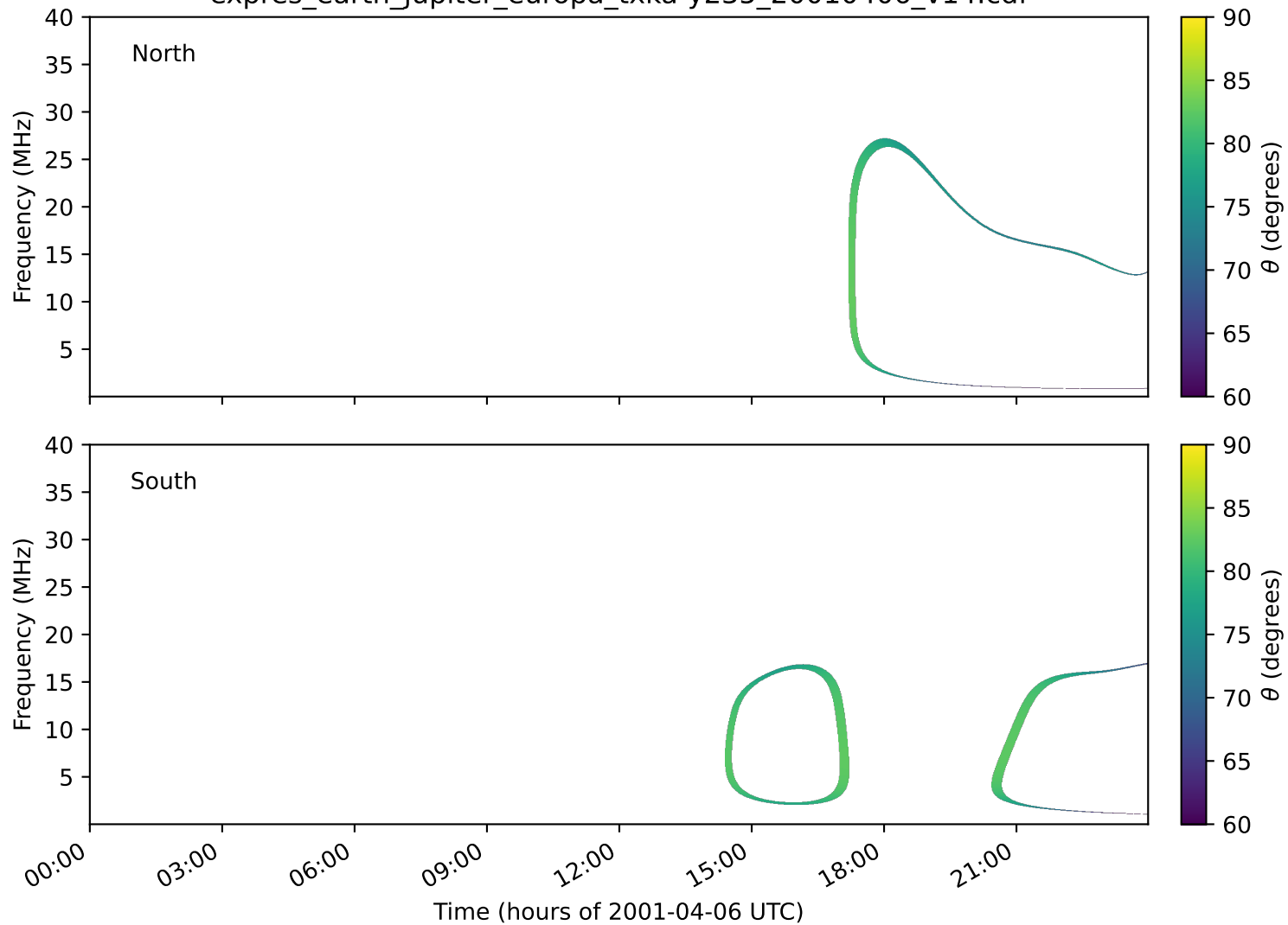
expres_earth_jupiter_europa_txka-y235_20010406_v14.cdf
