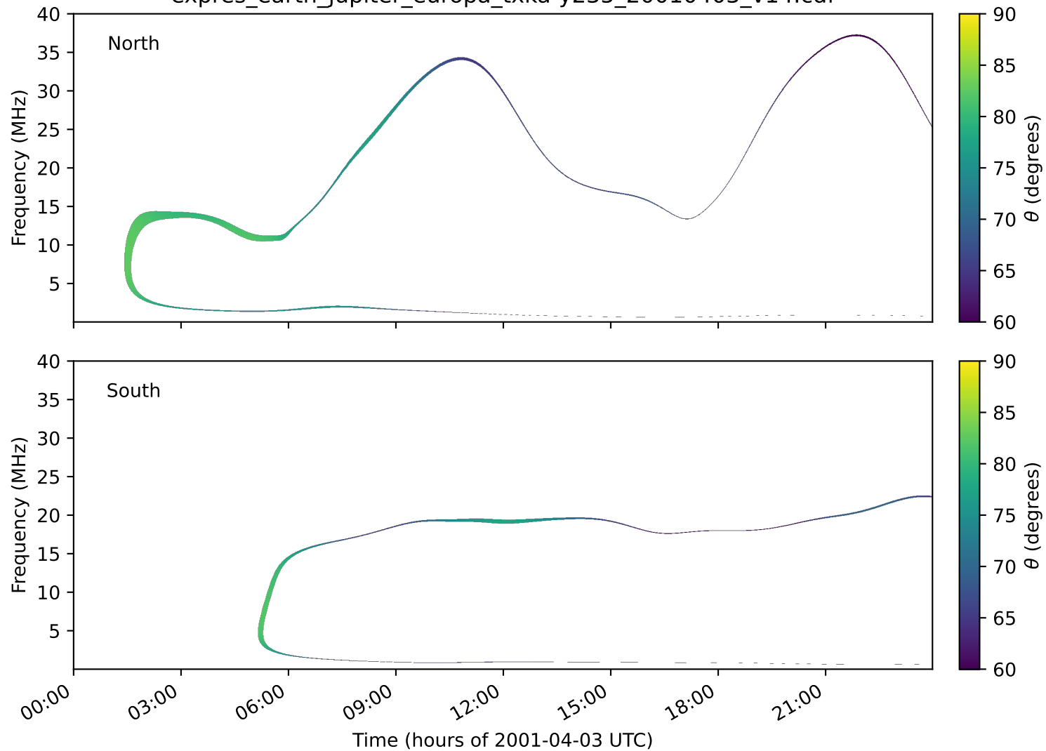
expres_earth_jupiter_europa_txka-y235_20010403_v14.cdf
