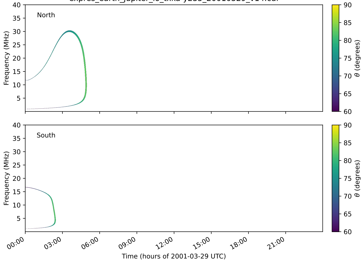
expres_earth_jupiter_io_txka-y235_20010329_v14.cdf
