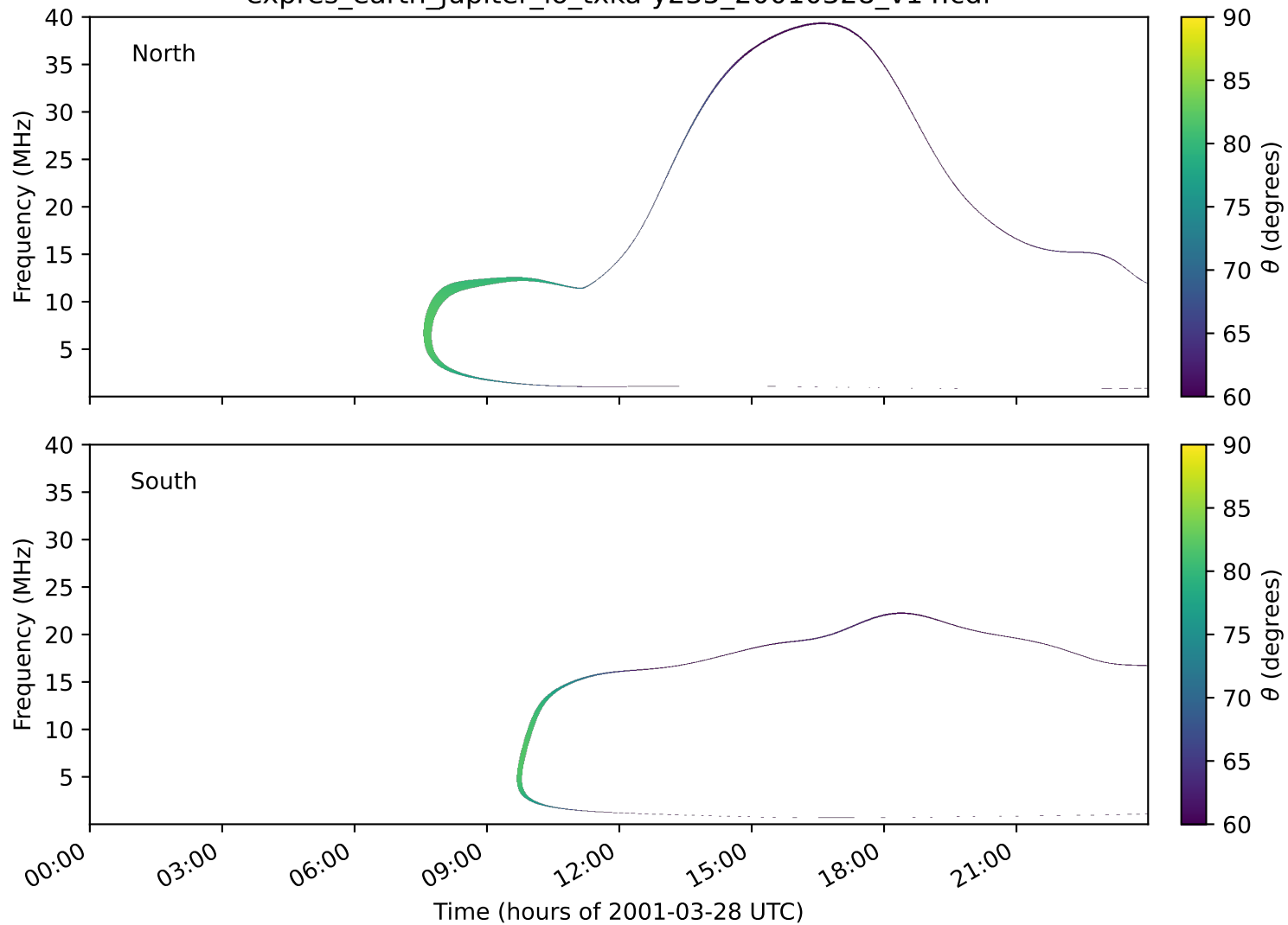
expres_earth_jupiter_io_txka-y235_20010328_v14.cdf
