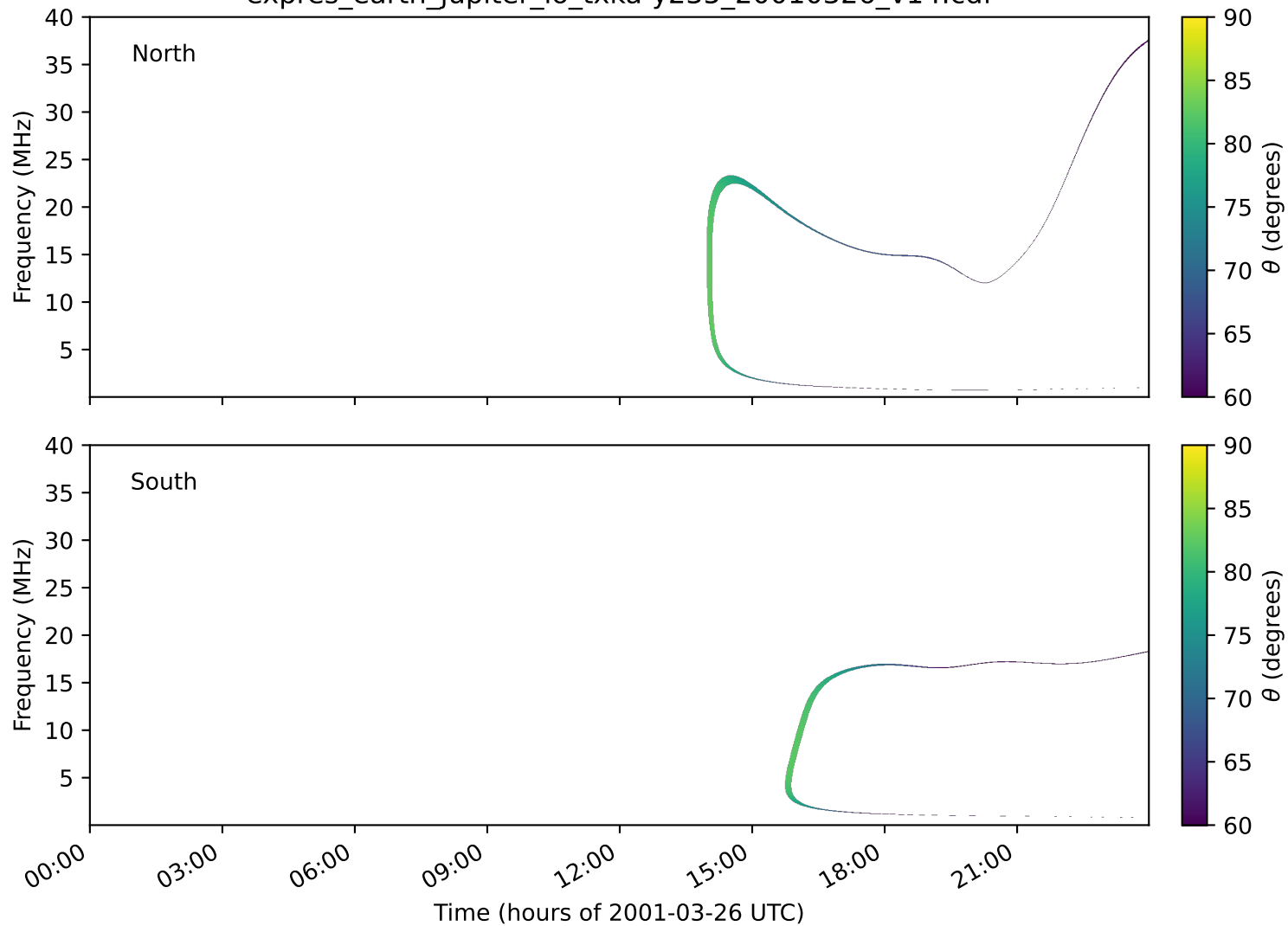
expres_earth_jupiter_io_txka-y235_20010326_v14.cdf
