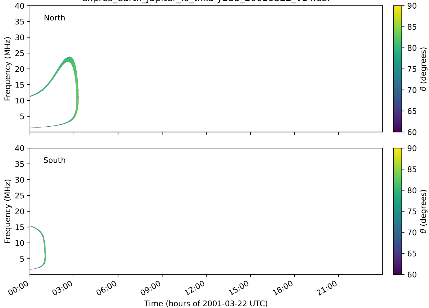
expres_earth_jupiter_io_txka-y235_20010322_v14.cdf
