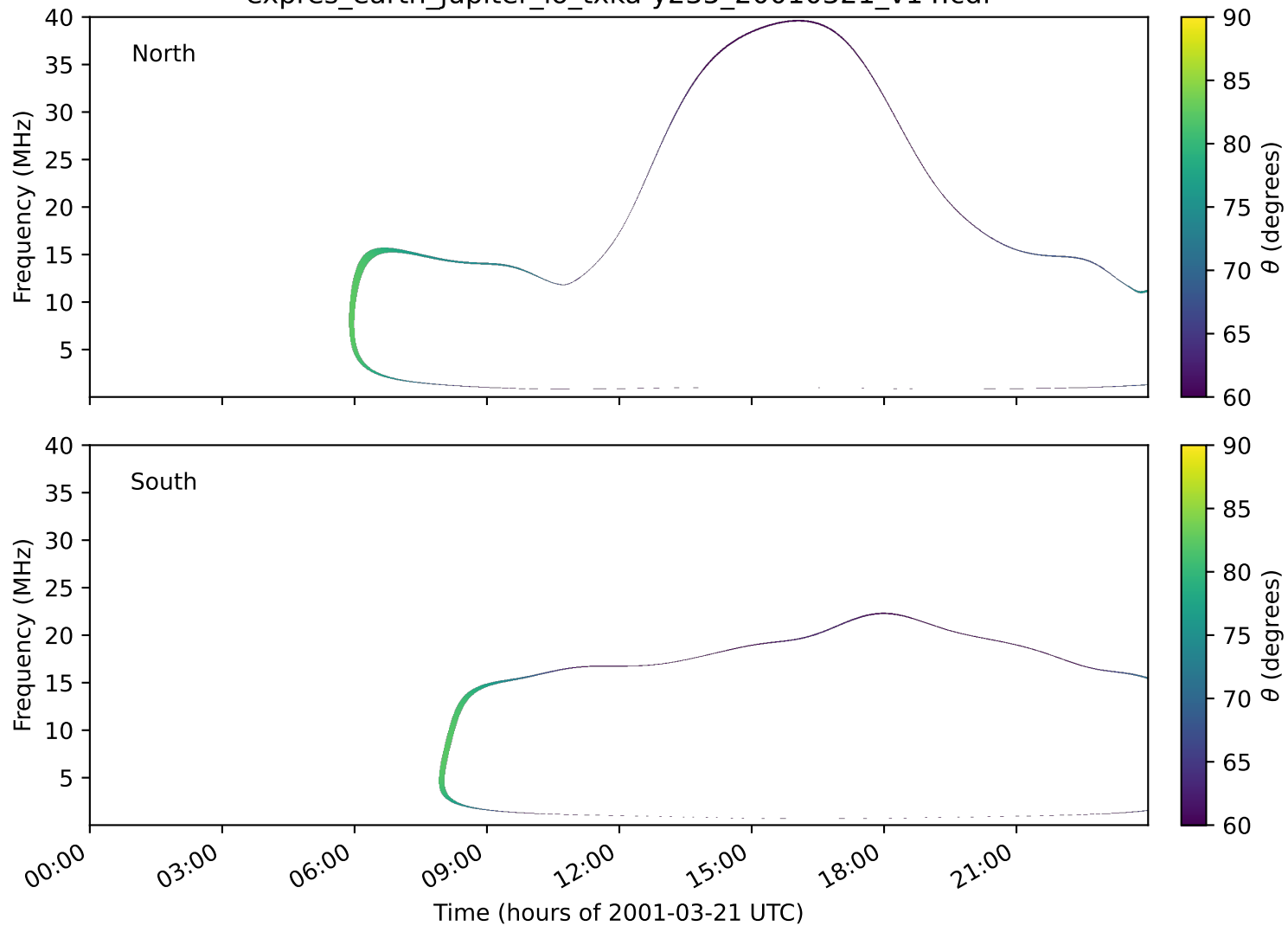
expres_earth_jupiter_io_txka-y235_20010321_v14.cdf
