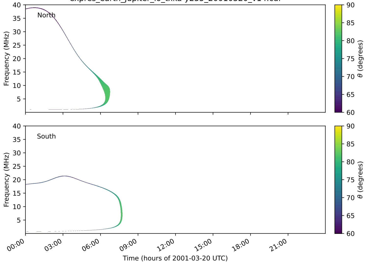
expres_earth_jupiter_io_txka-y235_20010320_v14.cdf
