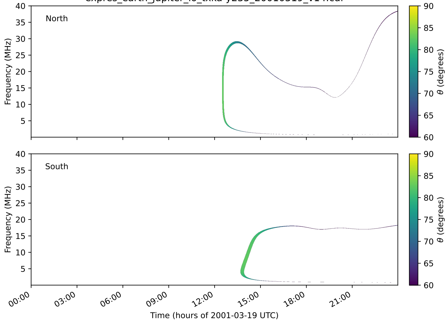
expres_earth_jupiter_io_txka-y235_20010319_v14.cdf
