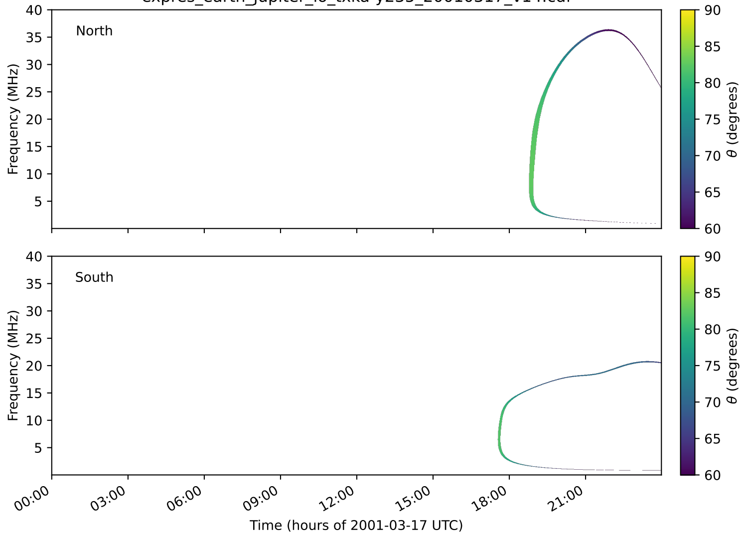
expres_earth_jupiter_io_txka-y235_20010317_v14.cdf
