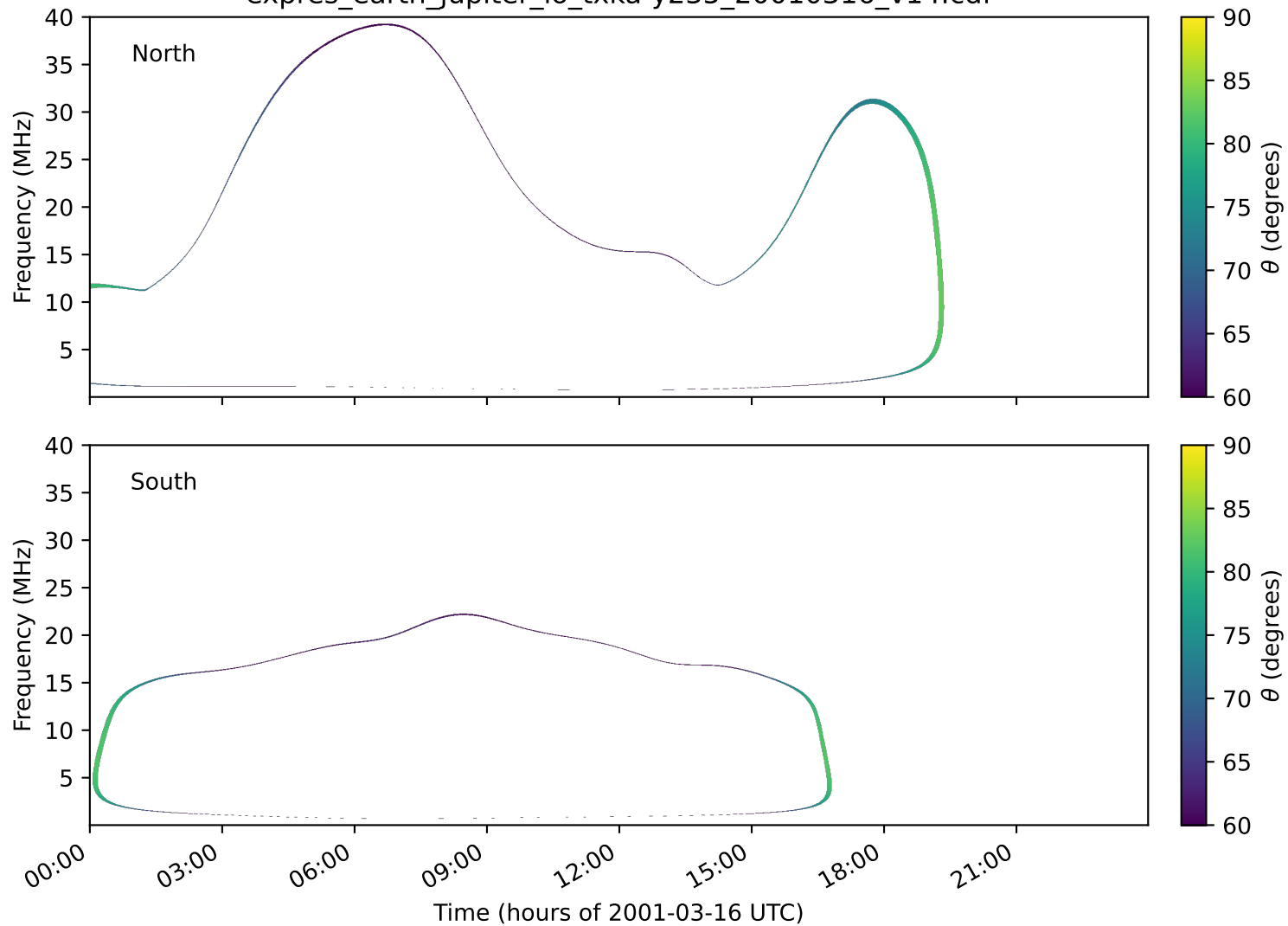
expres_earth_jupiter_io_txka-y235_20010316_v14.cdf
