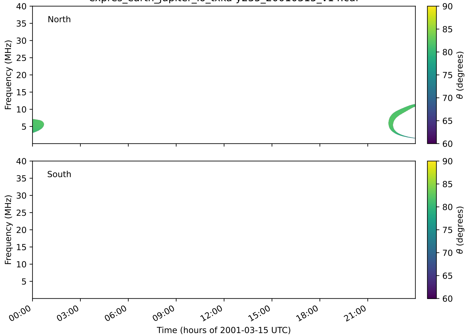
expres_earth_jupiter_io_txka-y235_20010315_v14.cdf
