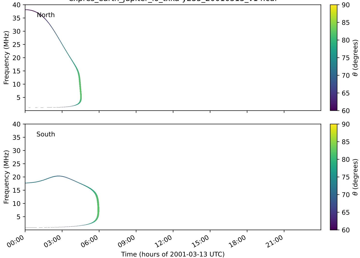
expres_earth_jupiter_io_txka-y235_20010313_v14.cdf
