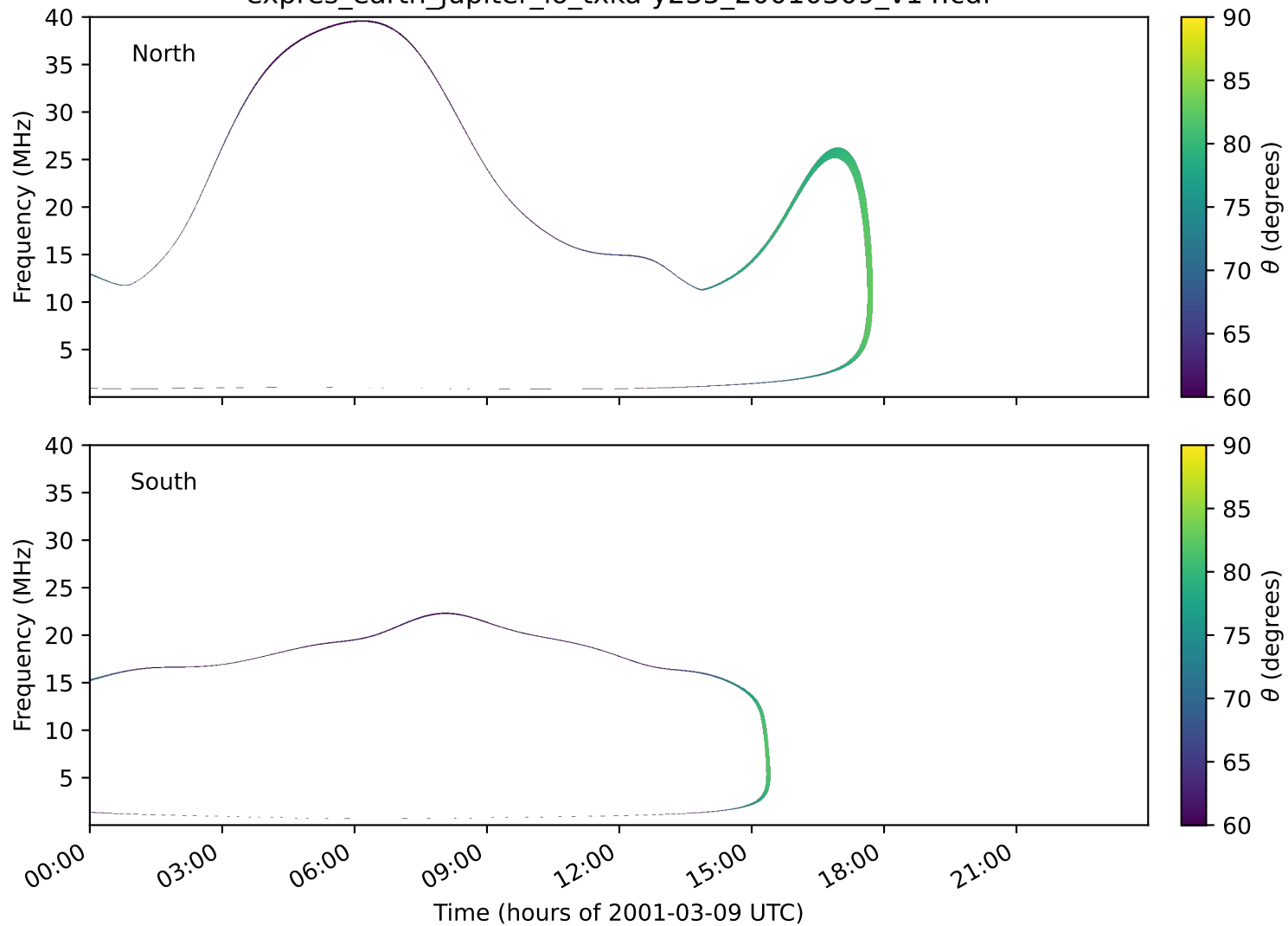
expres_earth_jupiter_io_txka-y235_20010309_v14.cdf
