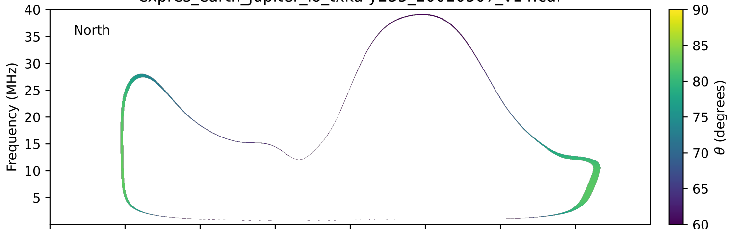
expres_earth_jupiter_io_txka-y235_20010307_v14.cdf
