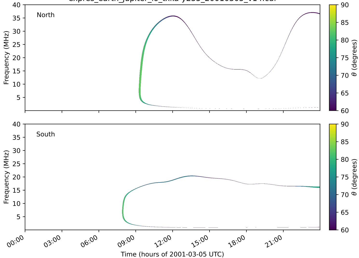
expres_earth_jupiter_io_txka-y235_20010305_v14.cdf
