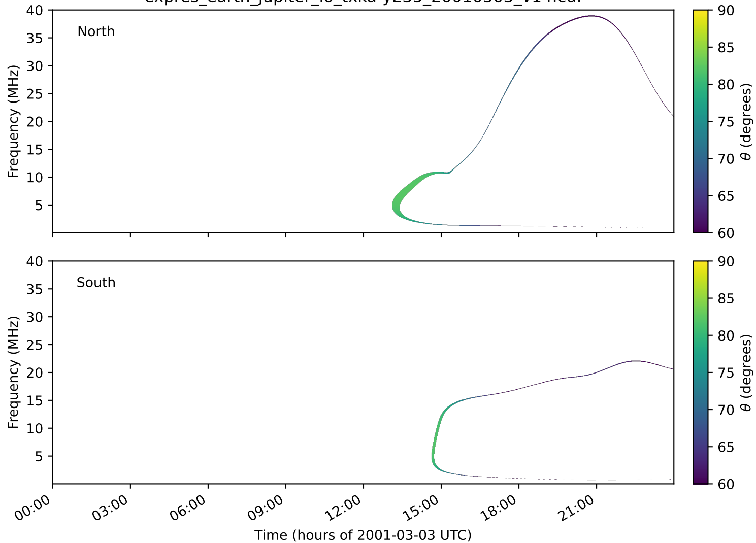
expres_earth_jupiter_io_txka-y235_20010303_v14.cdf
