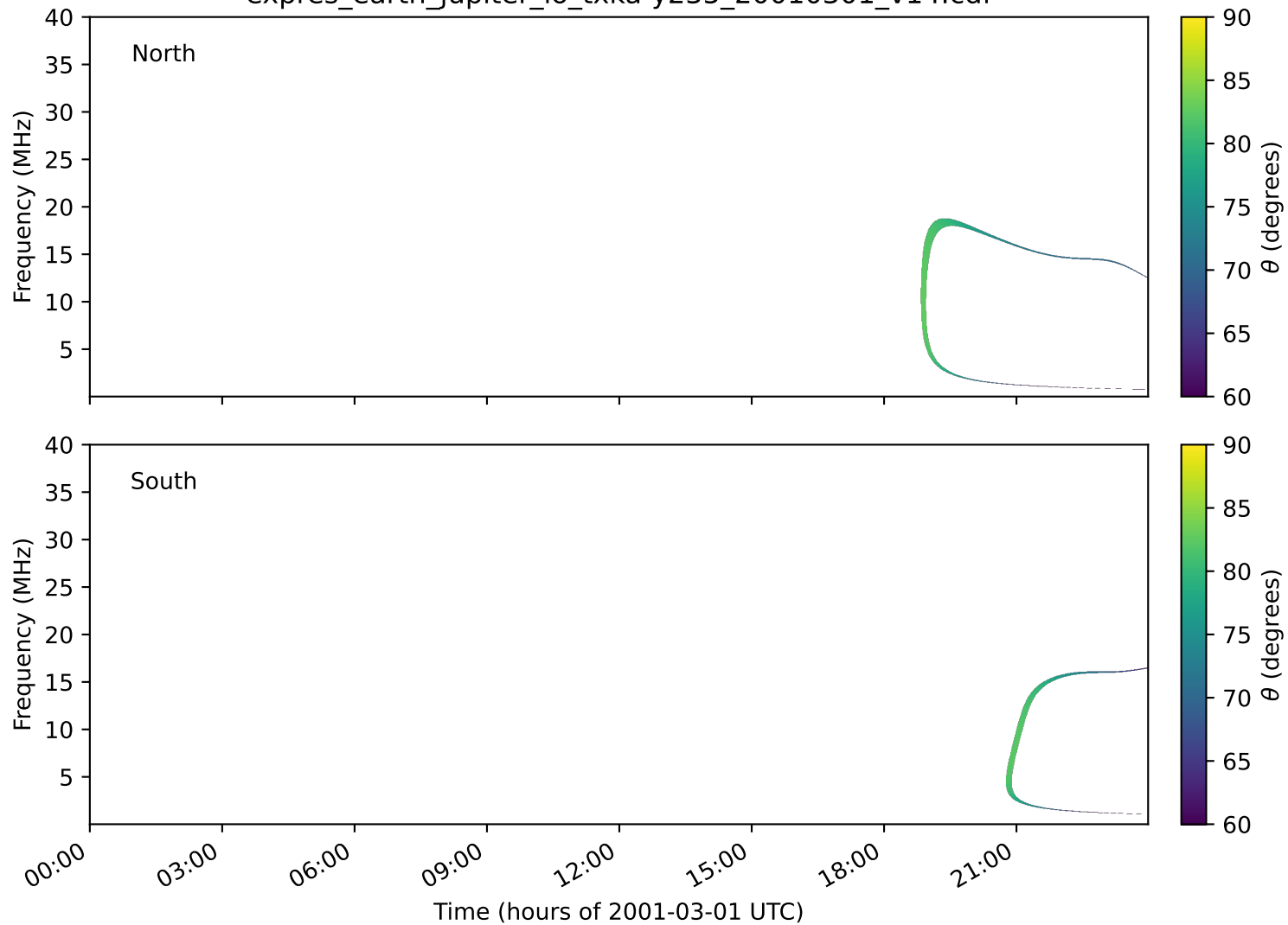
expres_earth_jupiter_io_txka-y235_20010301_v14.cdf
