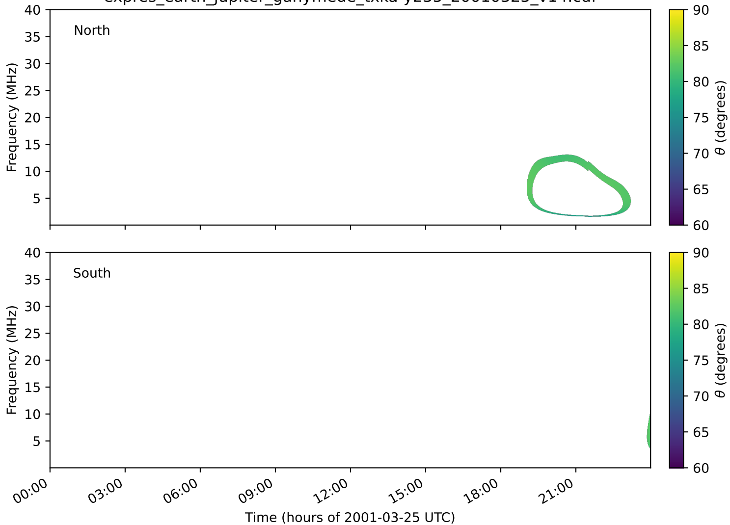
expres_earth_jupiter_ganymede_txka-y235_20010325_v14.cdf
