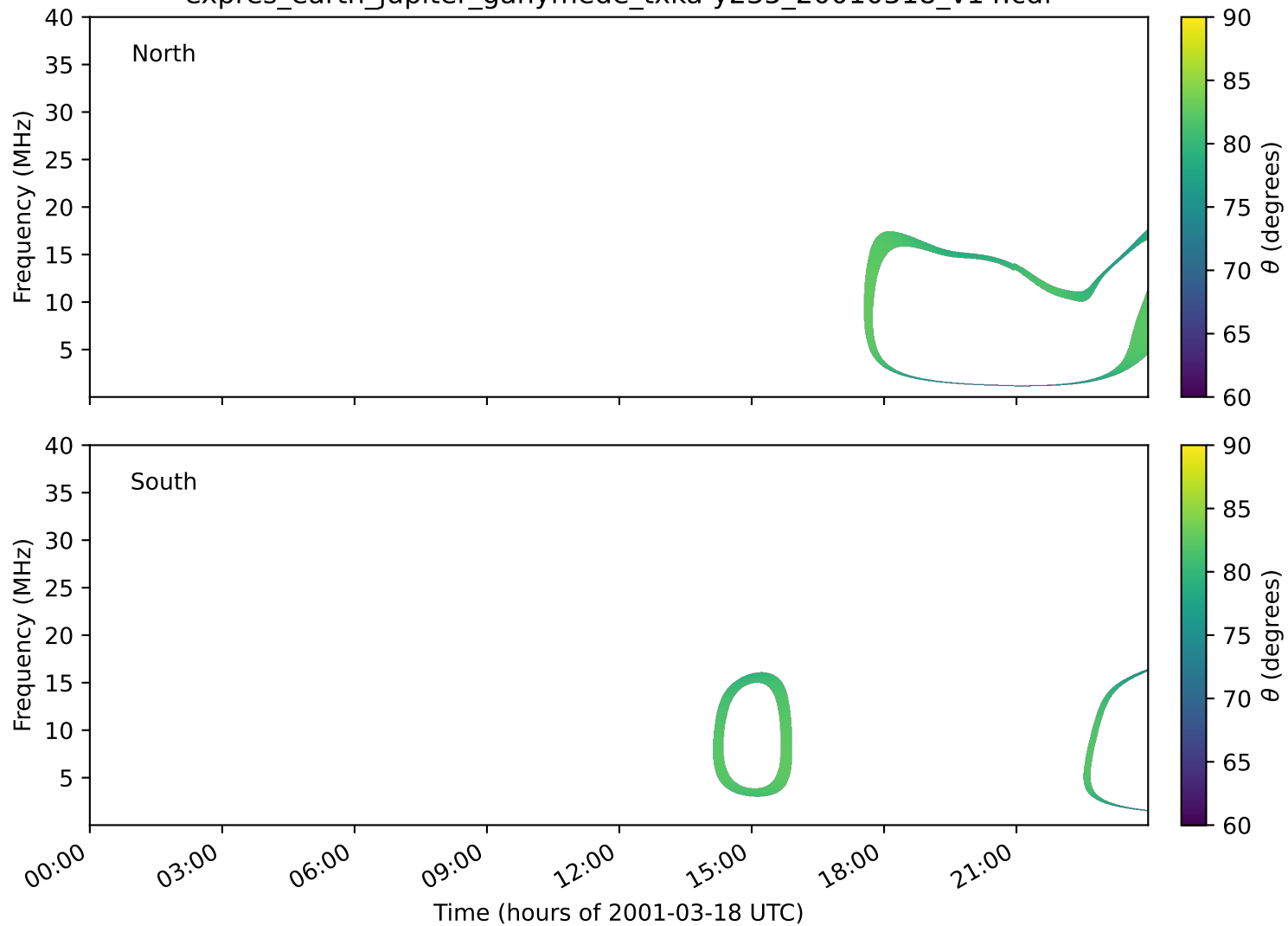
expres_earth_jupiter_ganymede_txka-y235_20010318_v14.cdf
