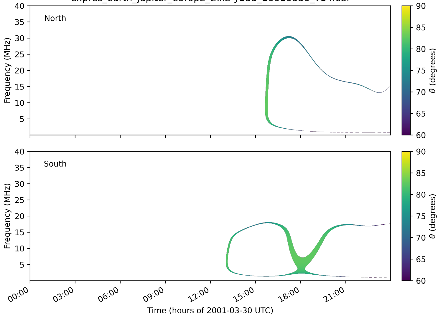
expres_earth_jupiter_europa_txka-y235_20010330_v14.cdf
