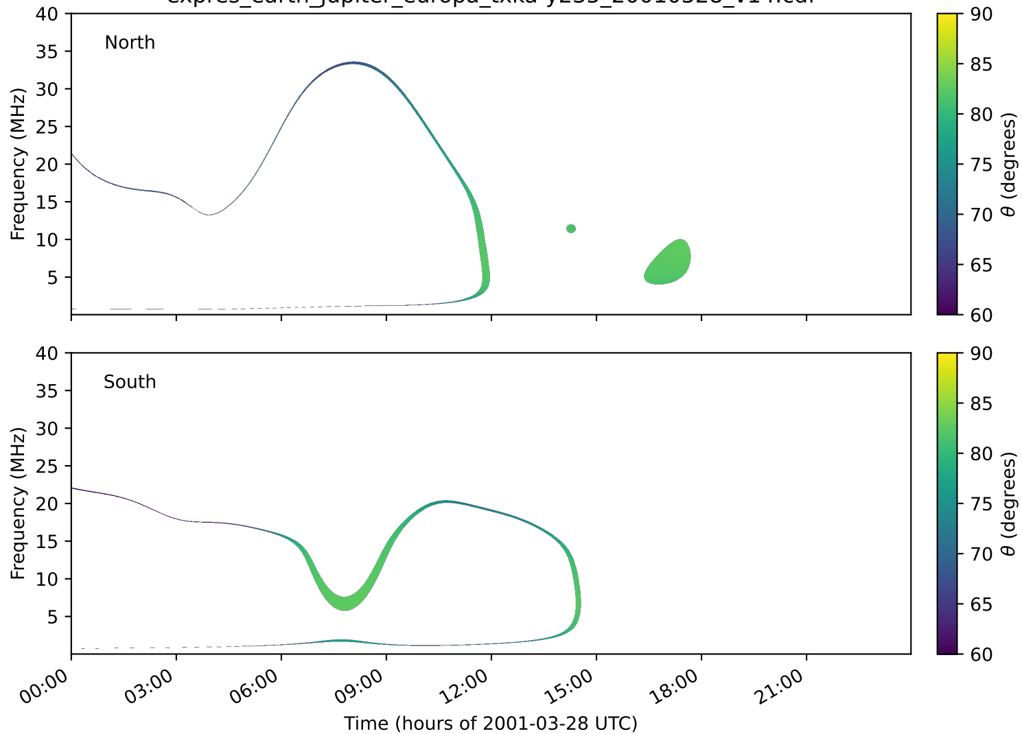
expres_earth_jupiter_europa_txka-y235_20010328_v14.cdf
