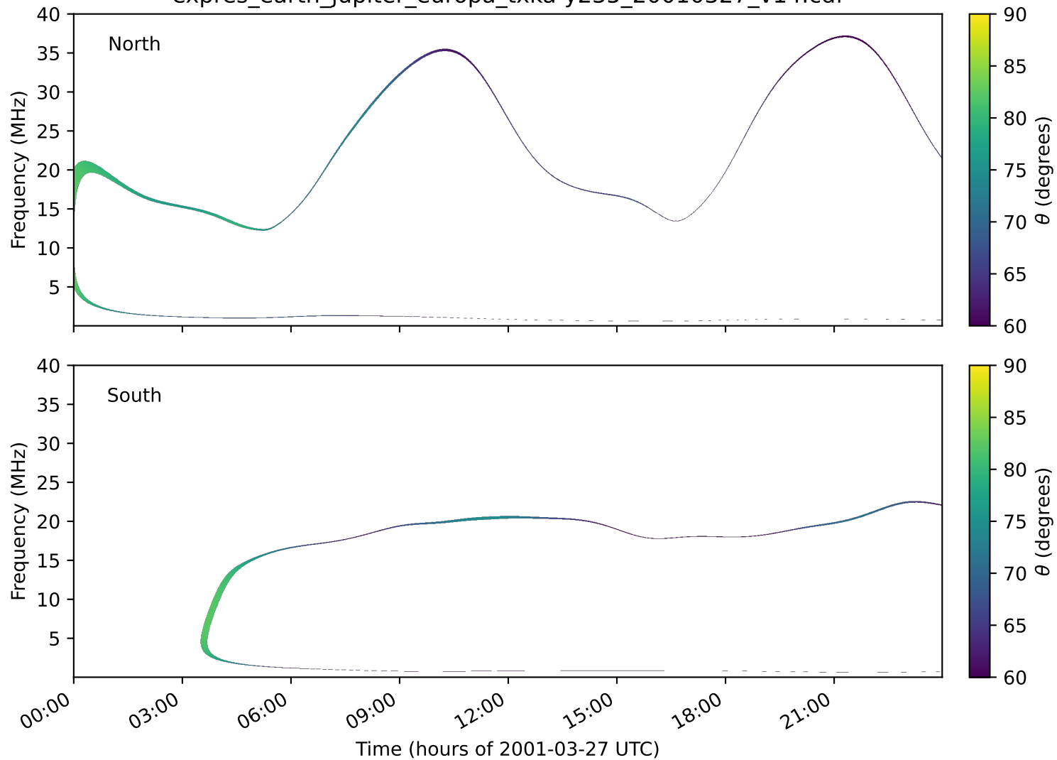
expres_earth_jupiter_europa_txka-y235_20010327_v14.cdf
