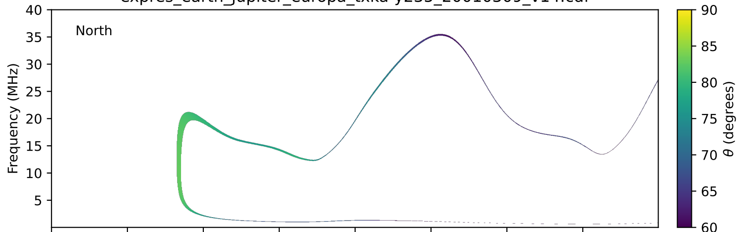
expres_earth_jupiter_europa_txka-y235_20010309_v14.cdf
