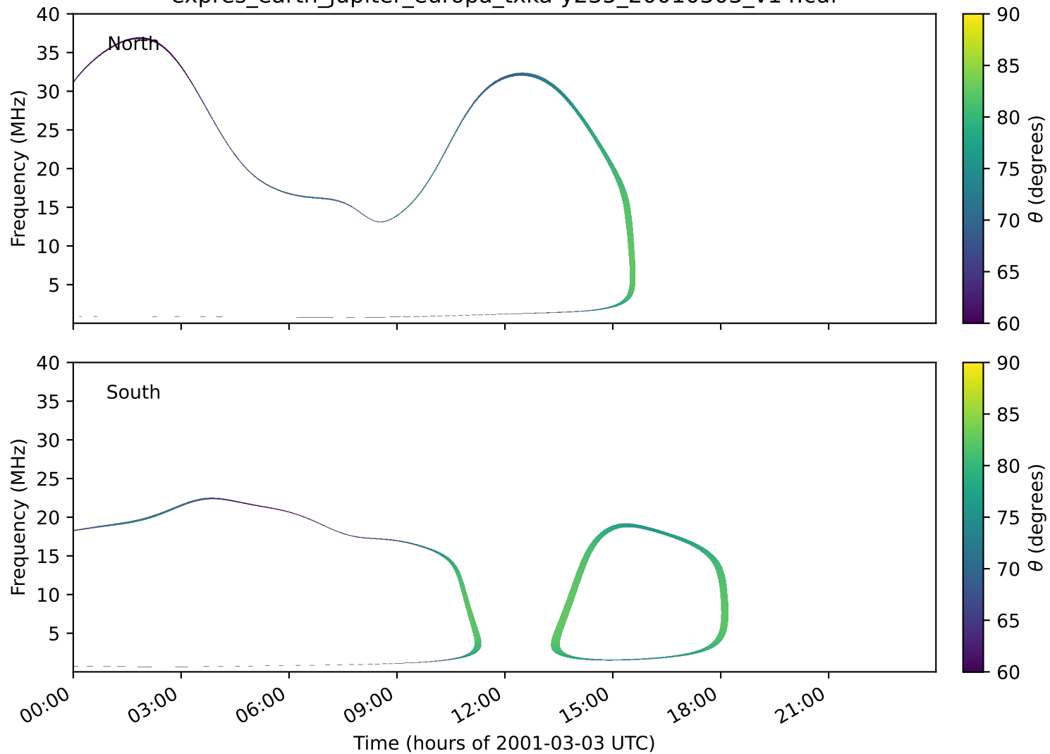
expres_earth_jupiter_europa_txka-y235_20010303_v14.cdf
