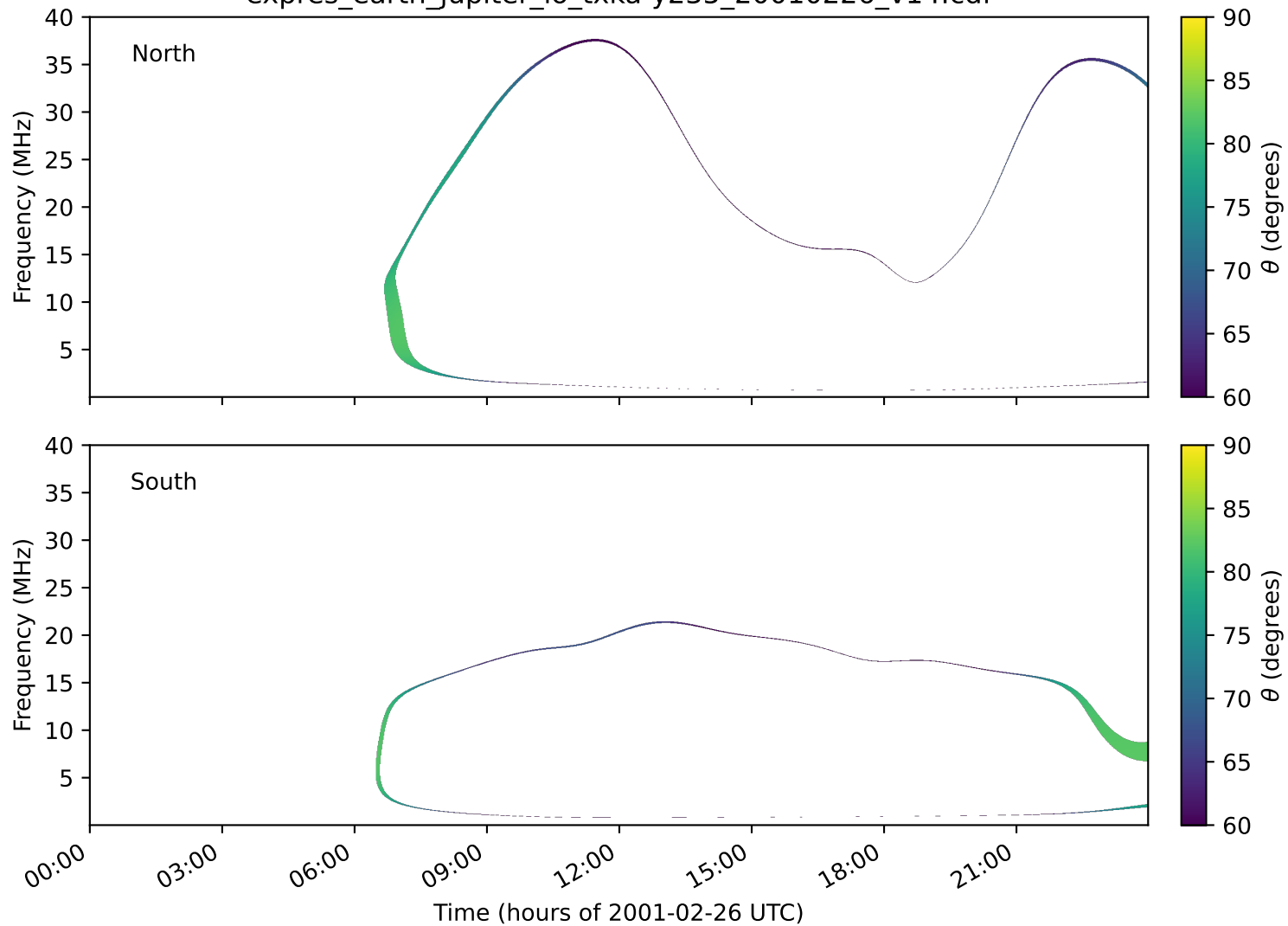
expres_earth_jupiter_io_txka-y235_20010226_v14.cdf
