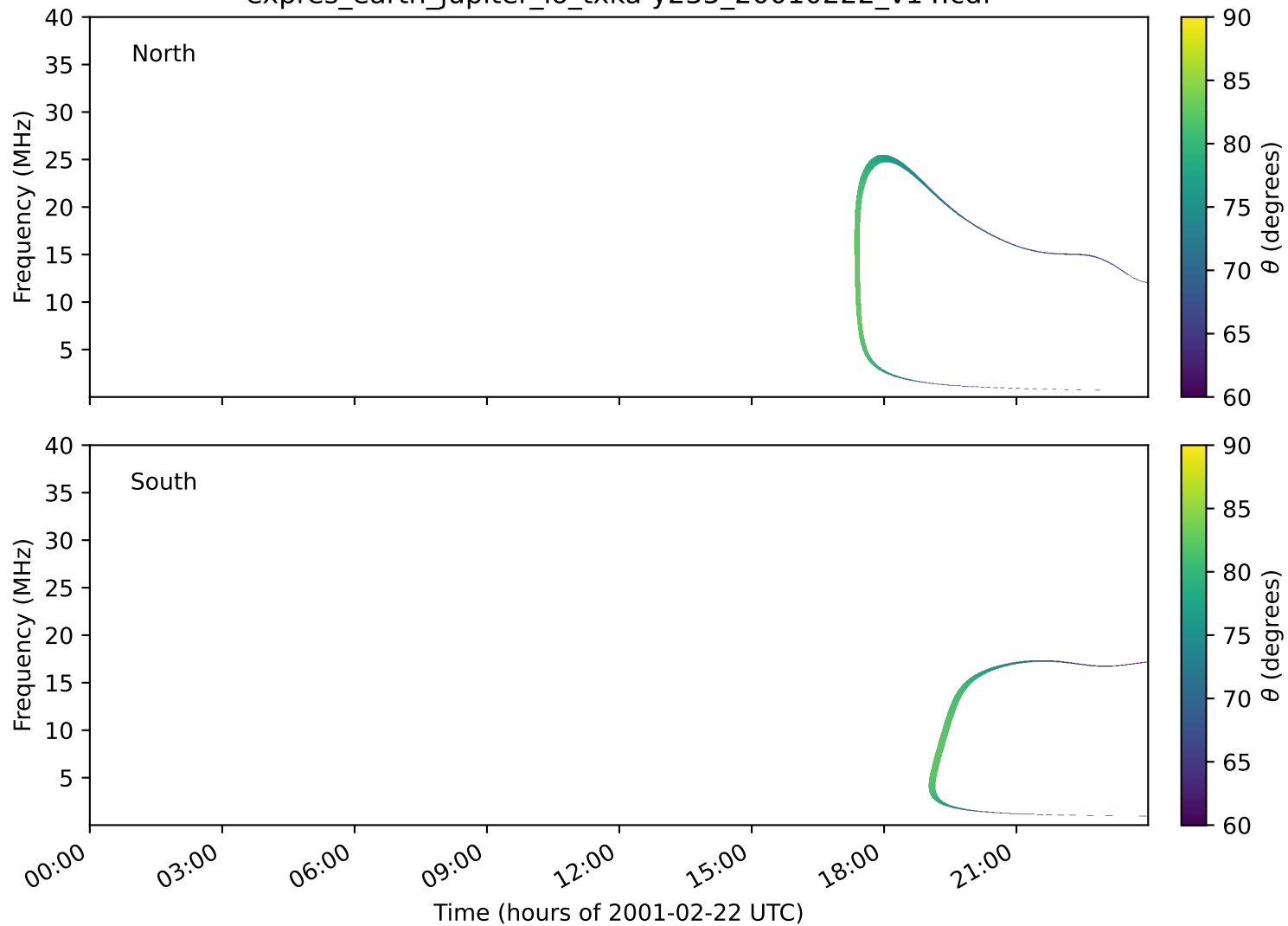
expres_earth_jupiter_io_txka-y235_20010222_v14.cdf
