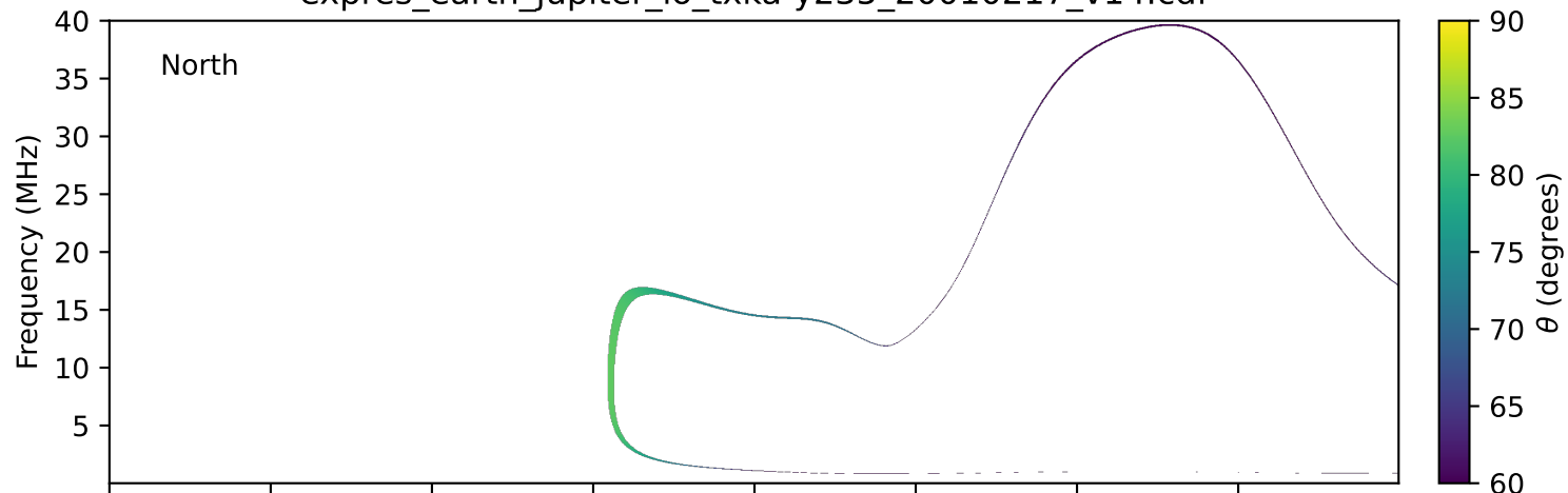
expres_earth_jupiter_io_txka-y235_20010217_v14.cdf
