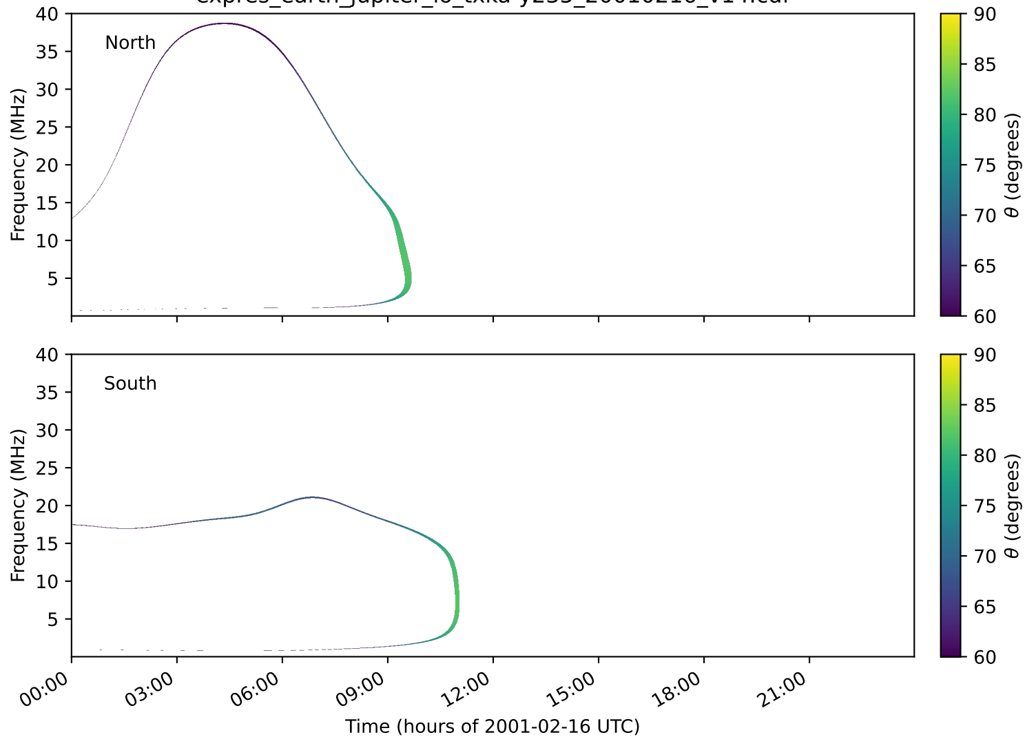
expres_earth_jupiter_io_txka-y235_20010216_v14.cdf
