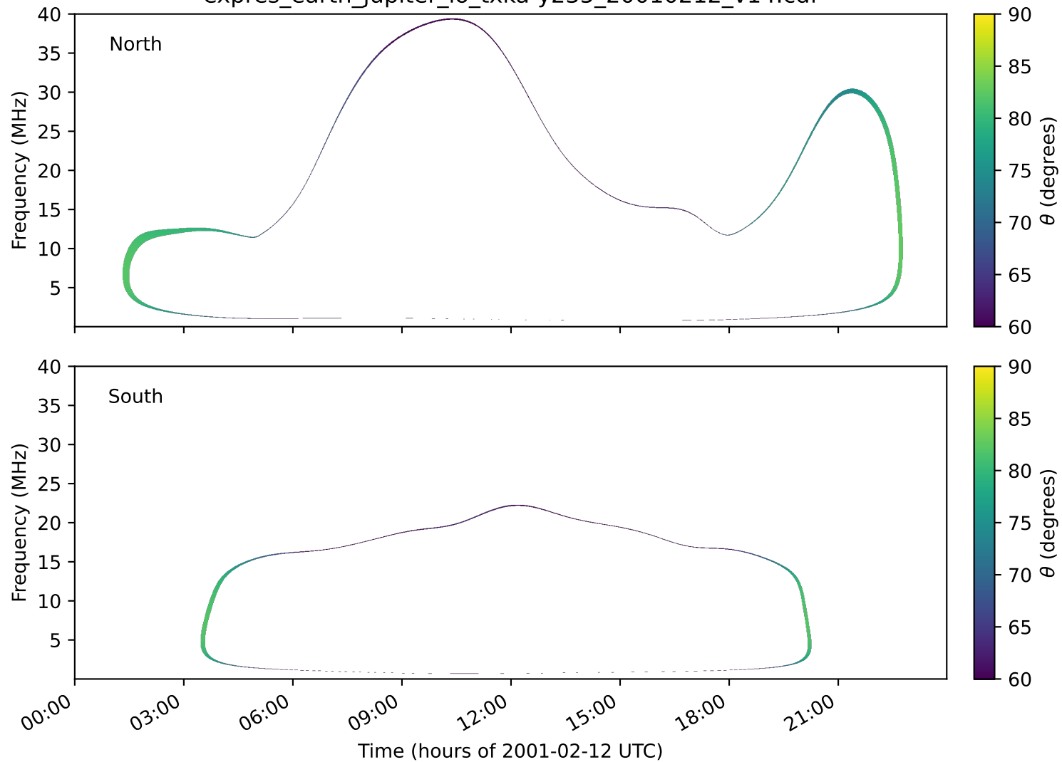
expres_earth_jupiter_io_txka-y235_20010212_v14.cdf
