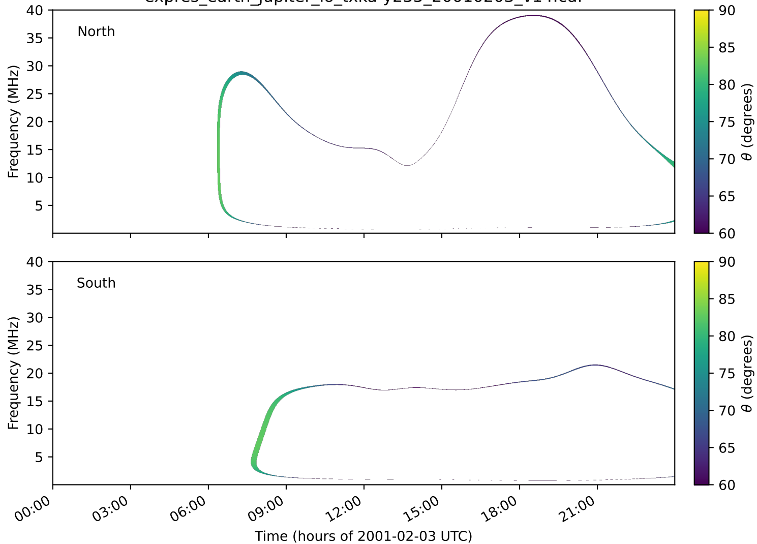
expres_earth_jupiter_io_txka-y235_20010203_v14.cdf
