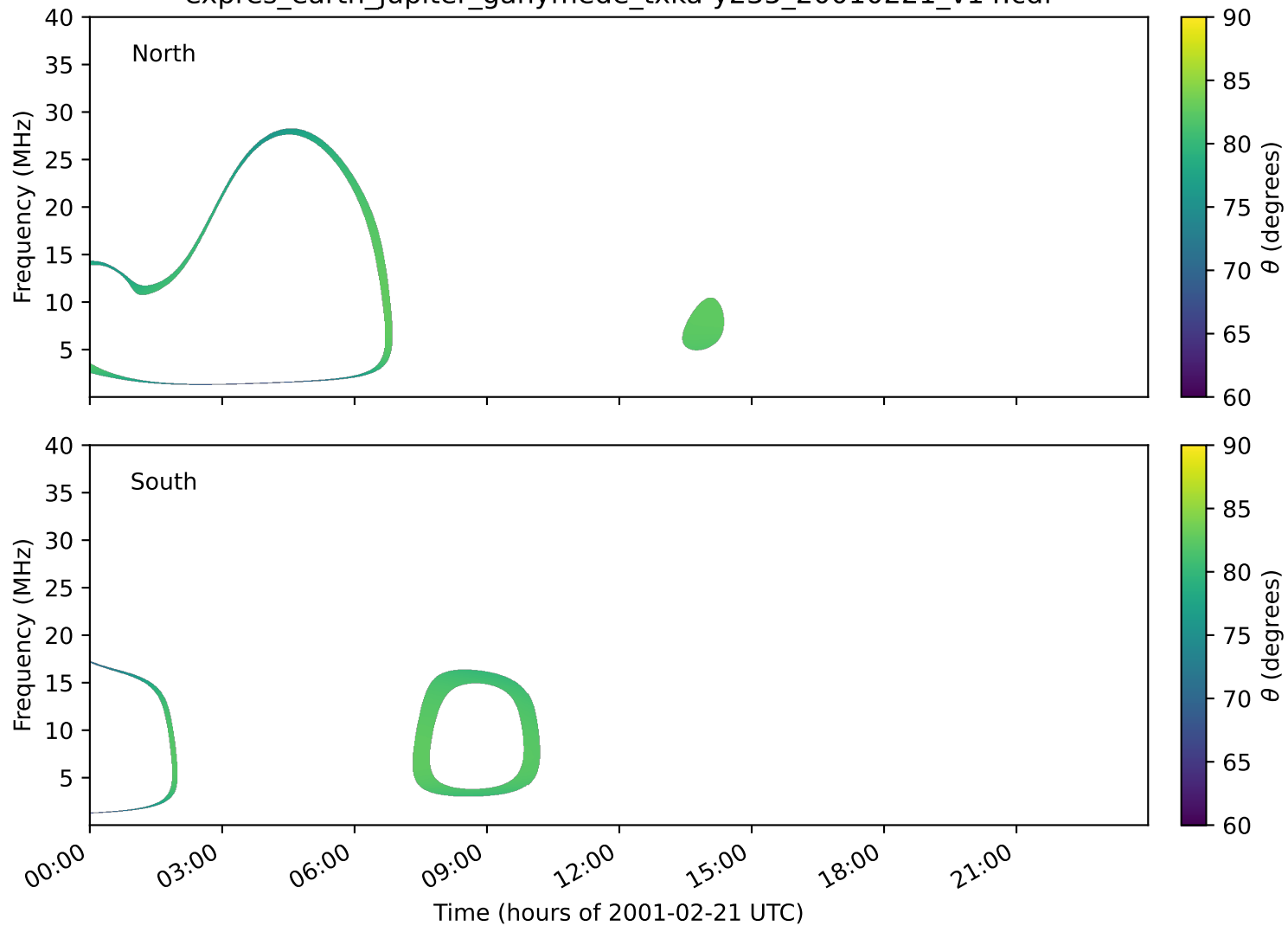
expres_earth_jupiter_ganymede_txka-y235_20010221_v14.cdf
