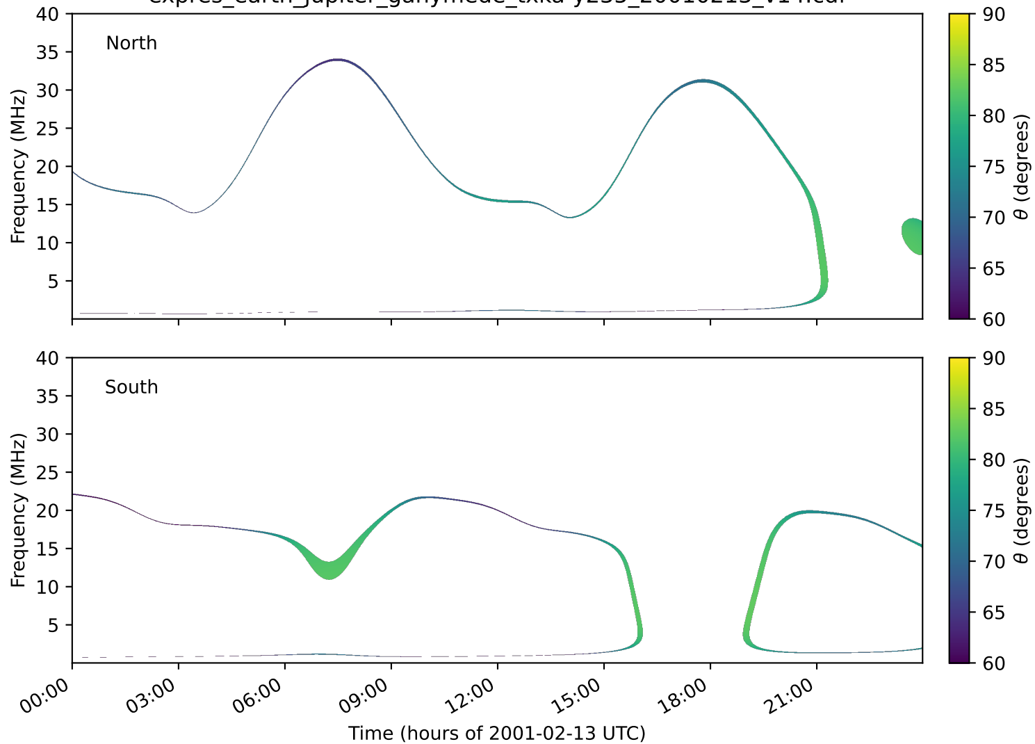
expres_earth_jupiter_ganymede_txka-y235_20010213_v14.cdf
