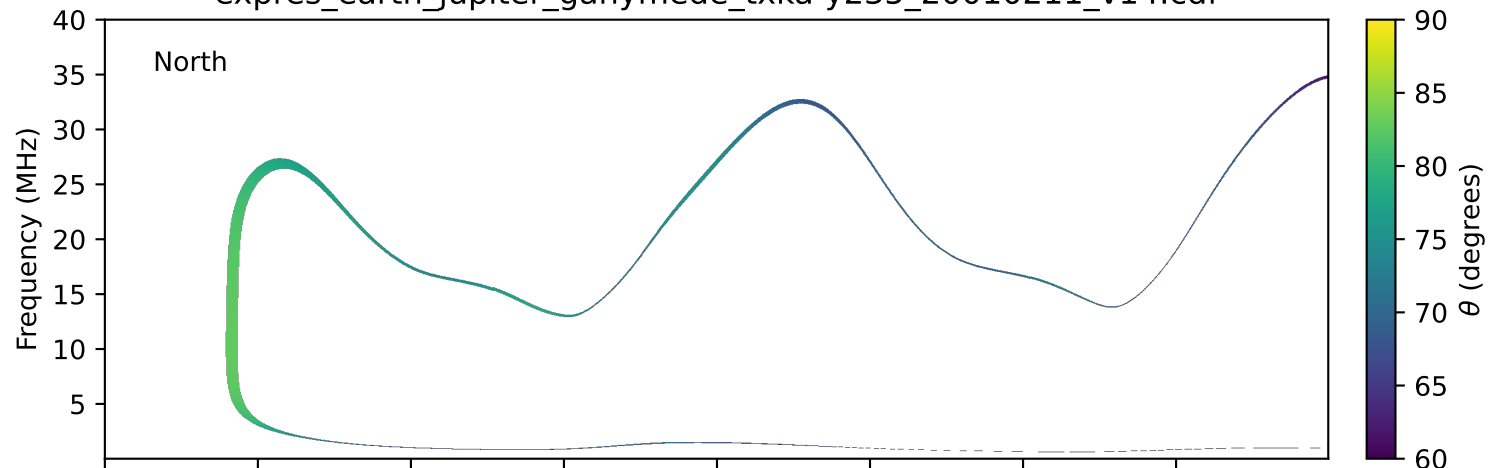
expres_earth_jupiter_ganymede_txka-y235_20010211_v14.cdf
