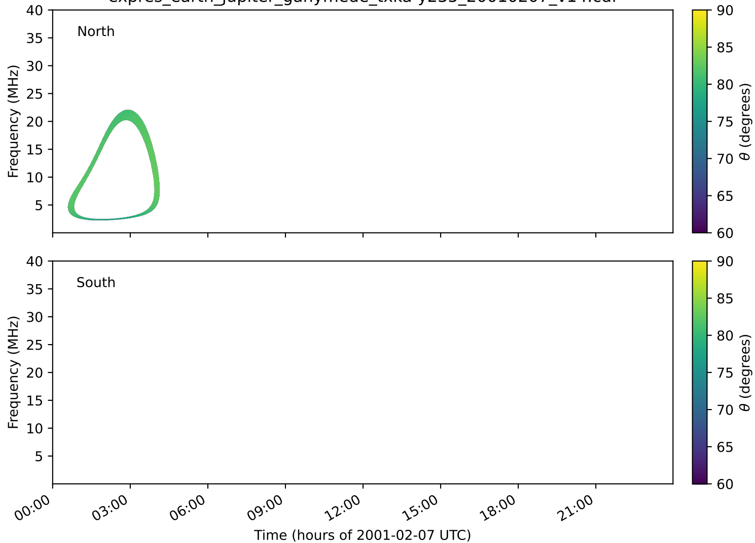
expres_earth_jupiter_ganymede_txka-y235_20010207_v14.cdf
