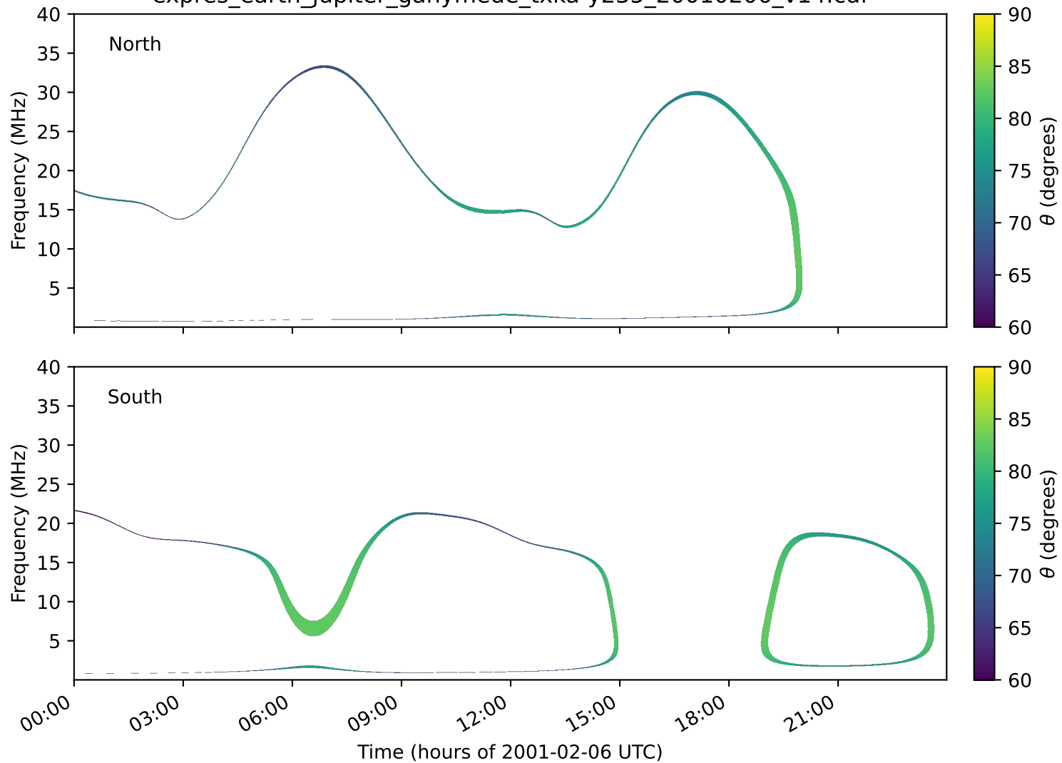
expres_earth_jupiter_ganymede_txka-y235_20010206_v14.cdf
