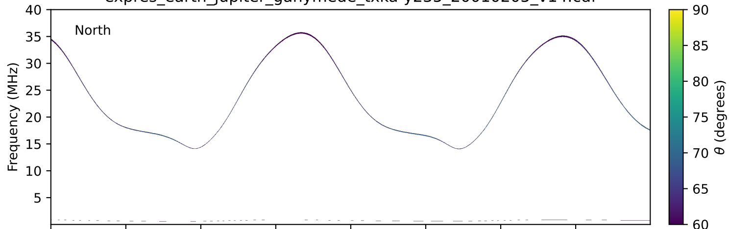
expres_earth_jupiter_ganymede_txka-y235_20010205_v14.cdf
