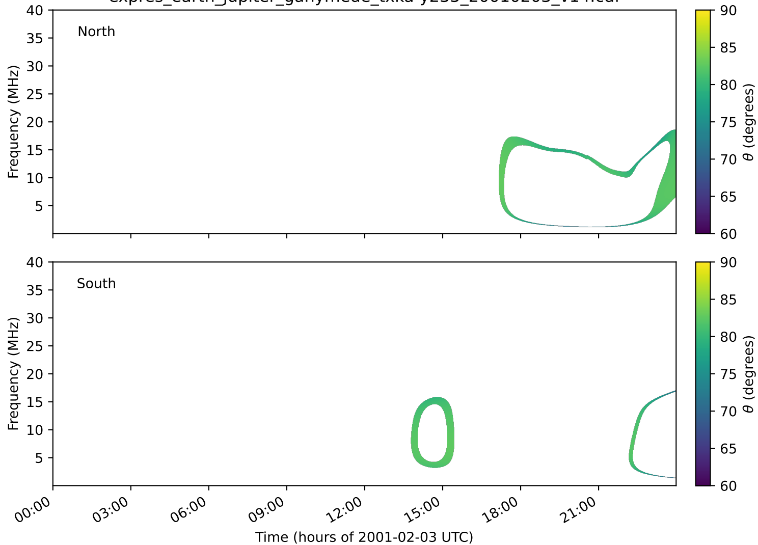
expres_earth_jupiter_ganymede_txka-y235_20010203_v14.cdf
