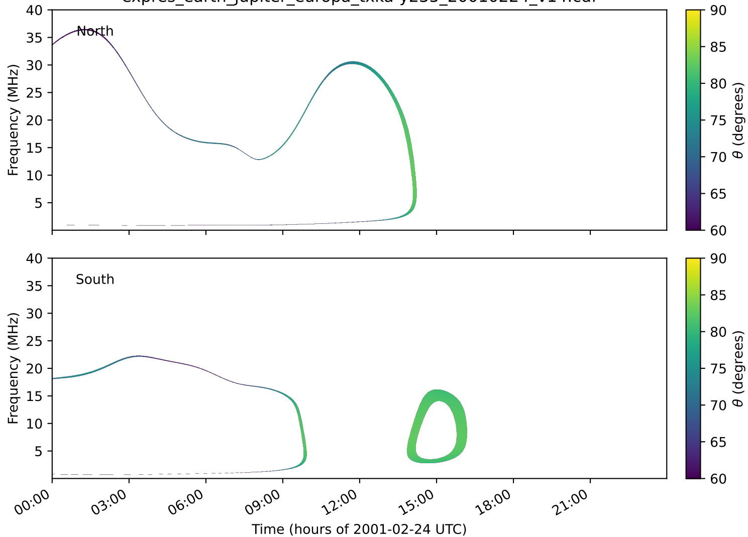
expres_earth_jupiter_europa_txka-y235_20010224_v14.cdf
