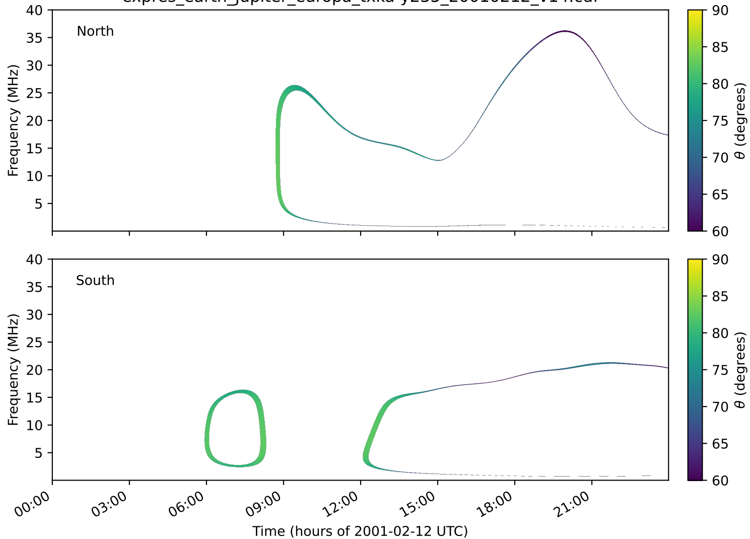
expres_earth_jupiter_europa_txka-y235_20010212_v14.cdf
