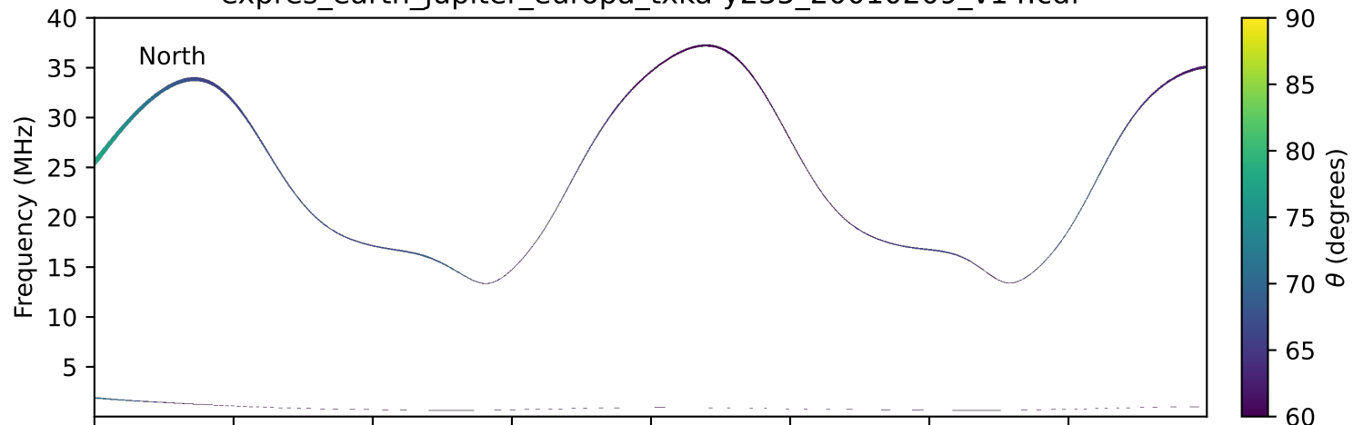
expres_earth_jupiter_europa_txka-y235_20010209_v14.cdf
