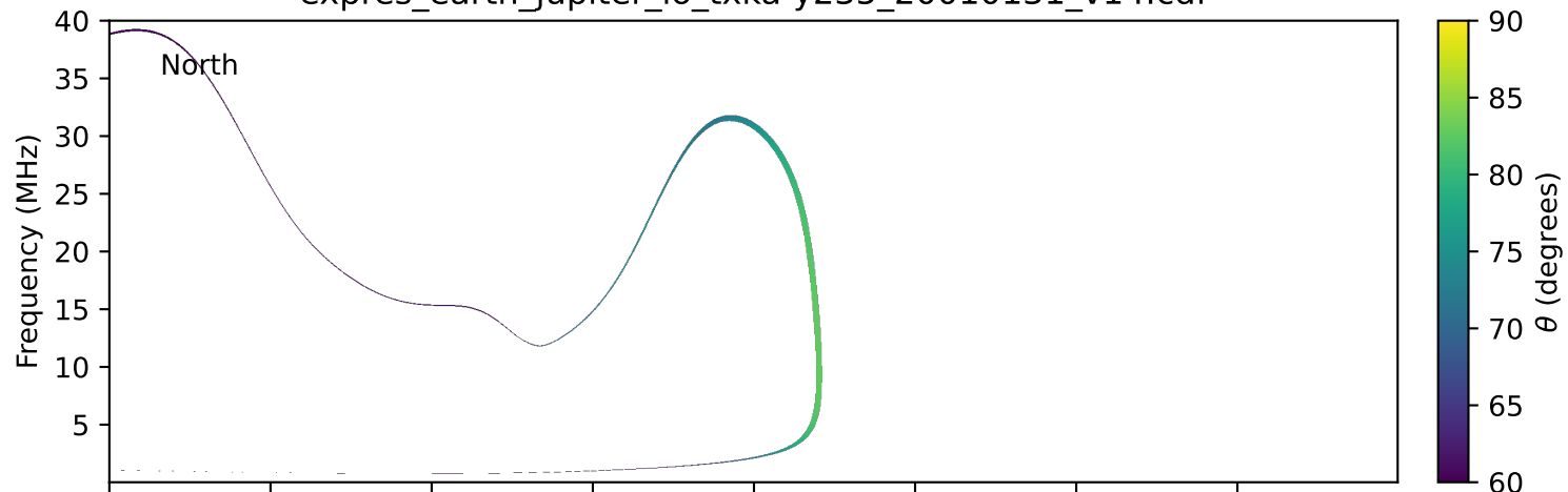
expres_earth_jupiter_io_txka-y235_20010131_v14.cdf
