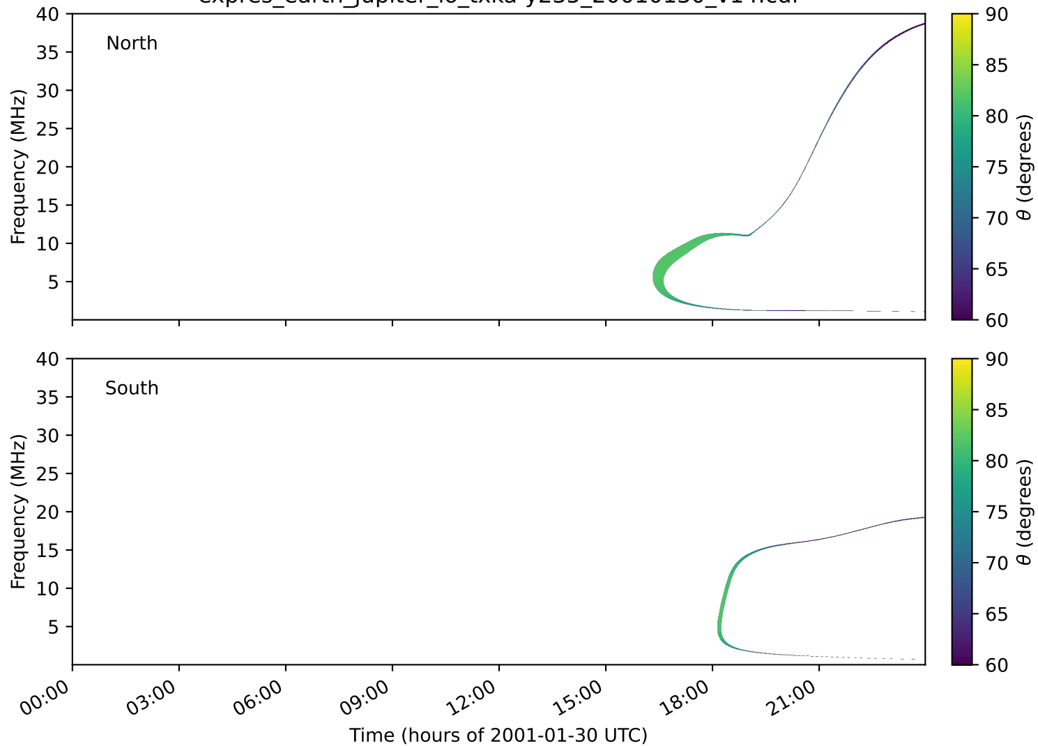
expres_earth_jupiter_io_txka-y235_20010130_v14.cdf
