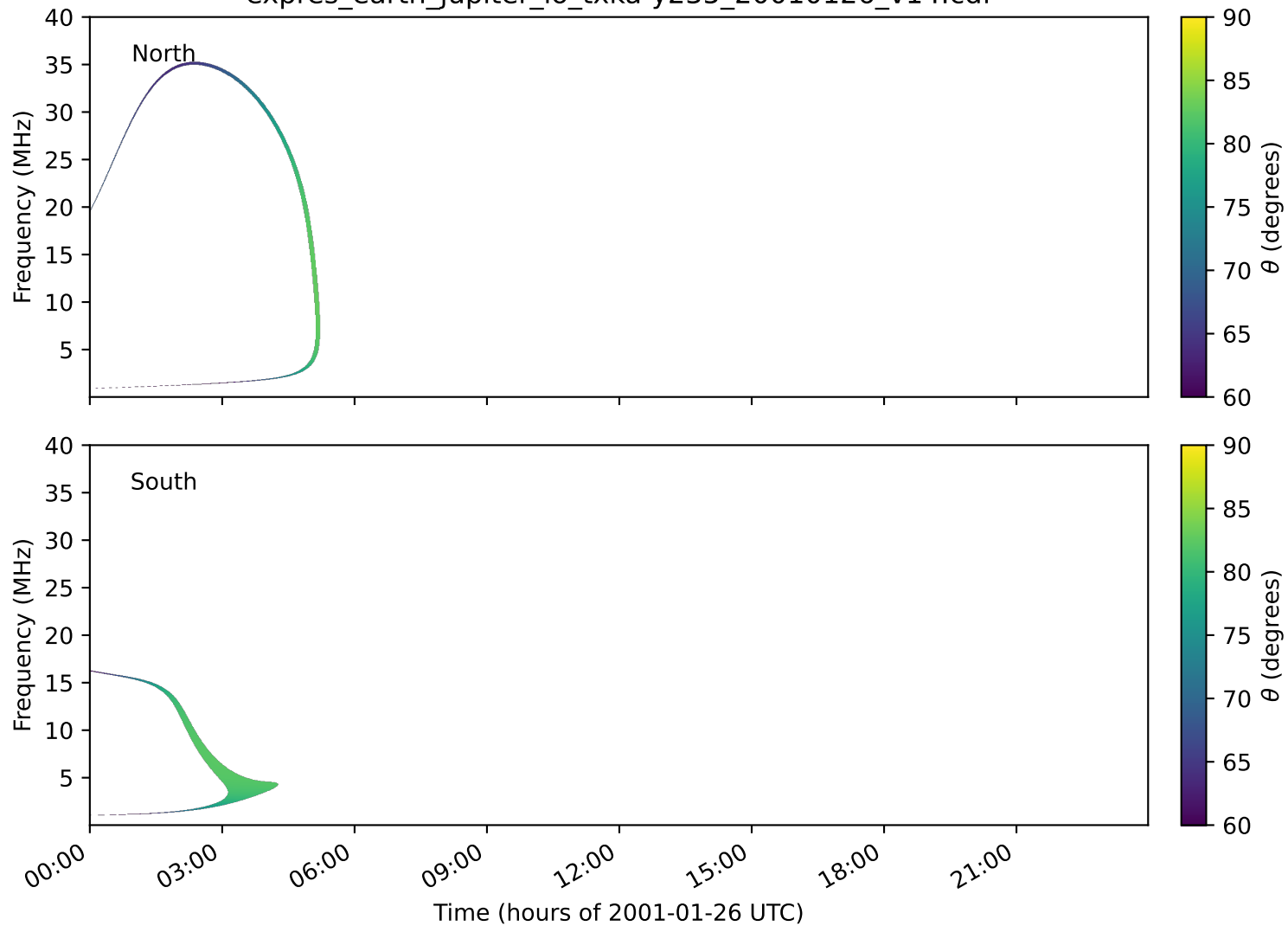
expres_earth_jupiter_io_txka-y235_20010126_v14.cdf
