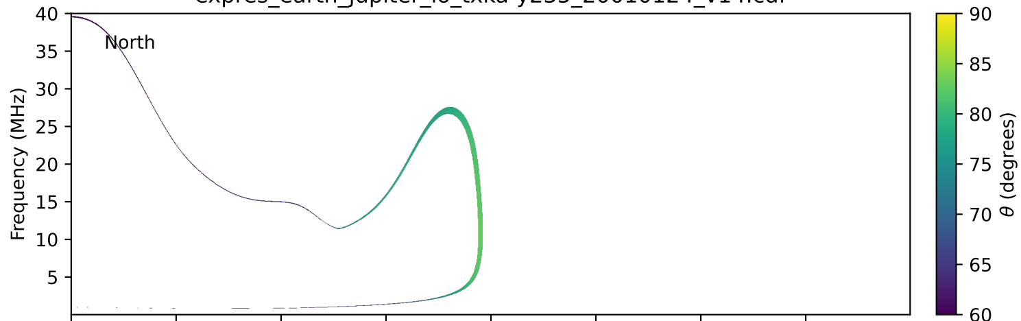
expres_earth_jupiter_io_txka-y235_20010124_v14.cdf
