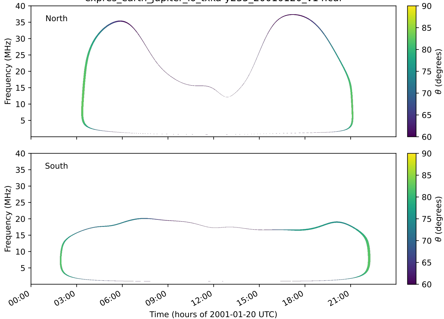
expres_earth_jupiter_io_txka-y235_20010120_v14.cdf
