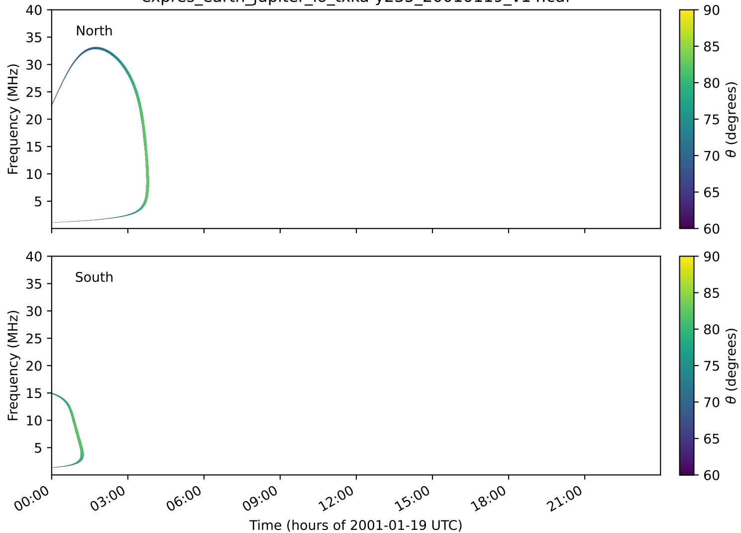
expres_earth_jupiter_io_txka-y235_20010119_v14.cdf
